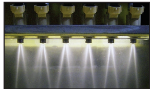
New Injectors
